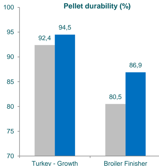
Pellet durability (%)
